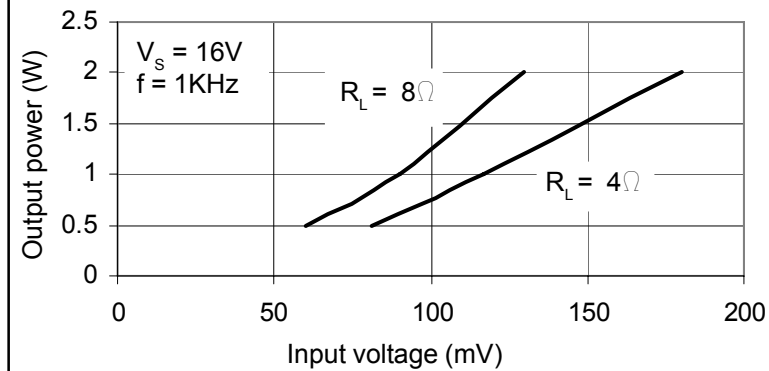
Figure 11. Sensitivity.
