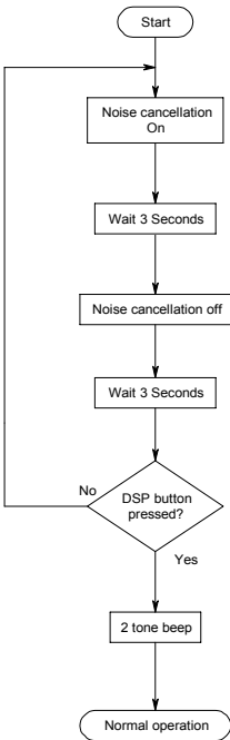
Figure 8. Demonstration modes.
