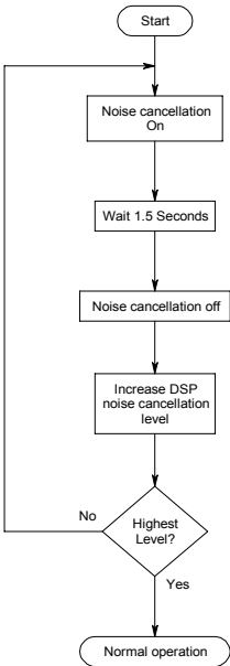
Figure 8. Demonstration modes.
