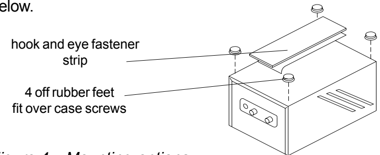
Figure 4. Mounting options
